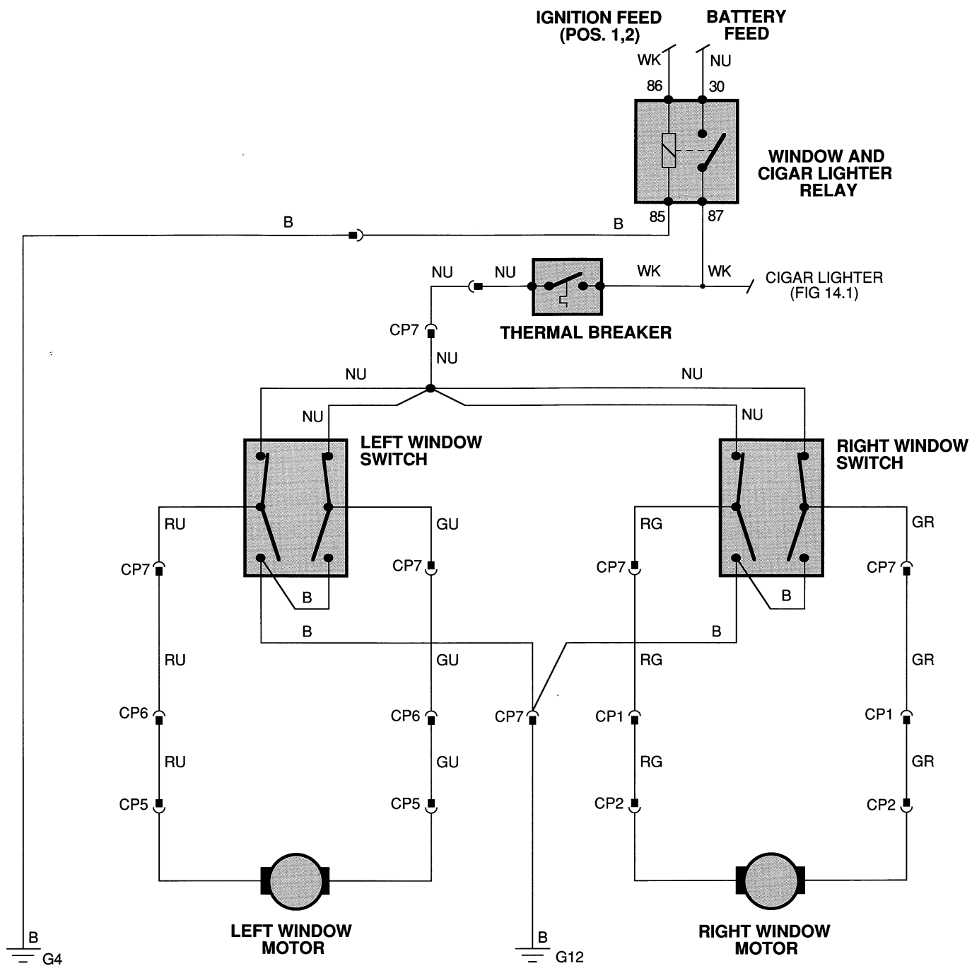
FIG 21.1 POWER WINDOWS XJ-S 1990 MY
