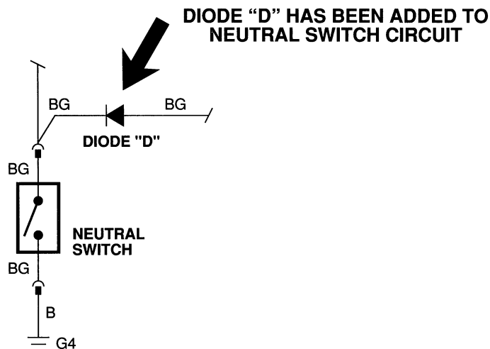
FIG 2.1 — BATTERY; STARTER; ALTERNATOR: WIRING DIAGRAM ADDITION
