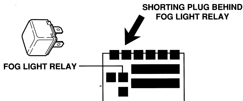
FIG 6.2 — FOG LIGHTS: COMPONENT LOCATION ADDITION
