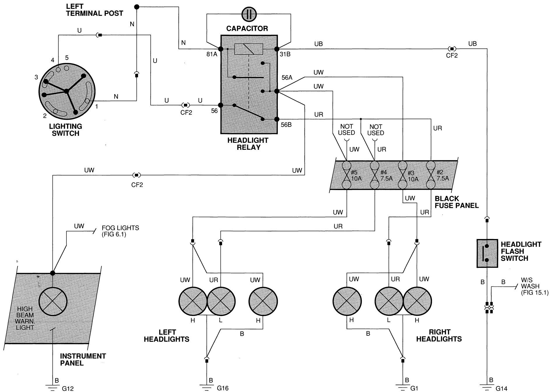
FIG 5.1 HEADLIGHTS XJ-S 1990 MY
